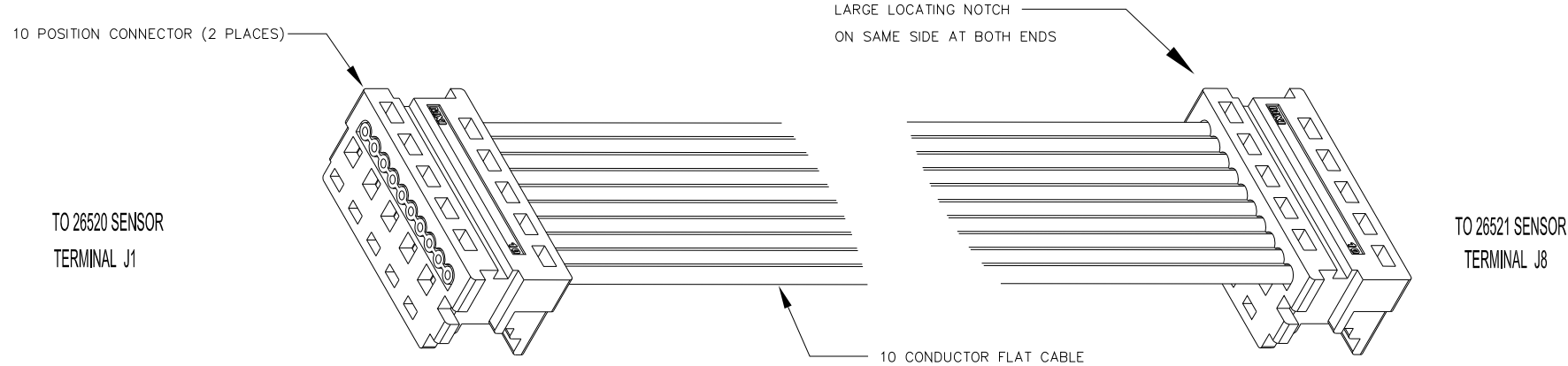
21426 HARNESS, DELIVERY SENSOR DETECTOR/EMITTER
