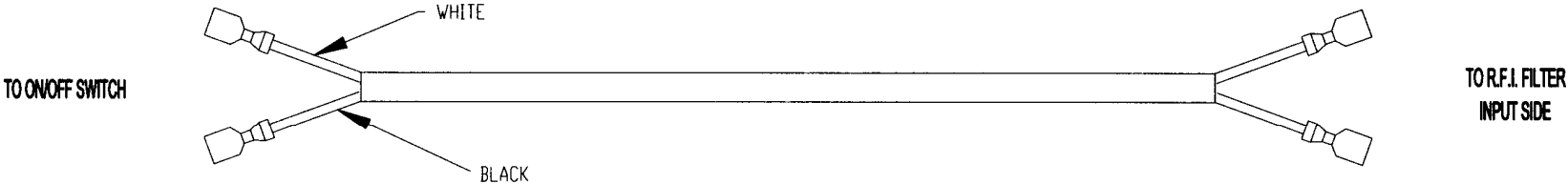
21485, HARNESS, ON/OFF SWITCH
