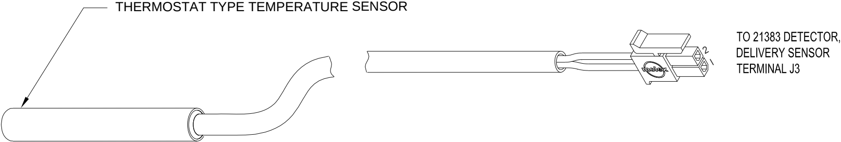
21468 THERMOSTAT TYPE TEMPERATURE SENSOR
