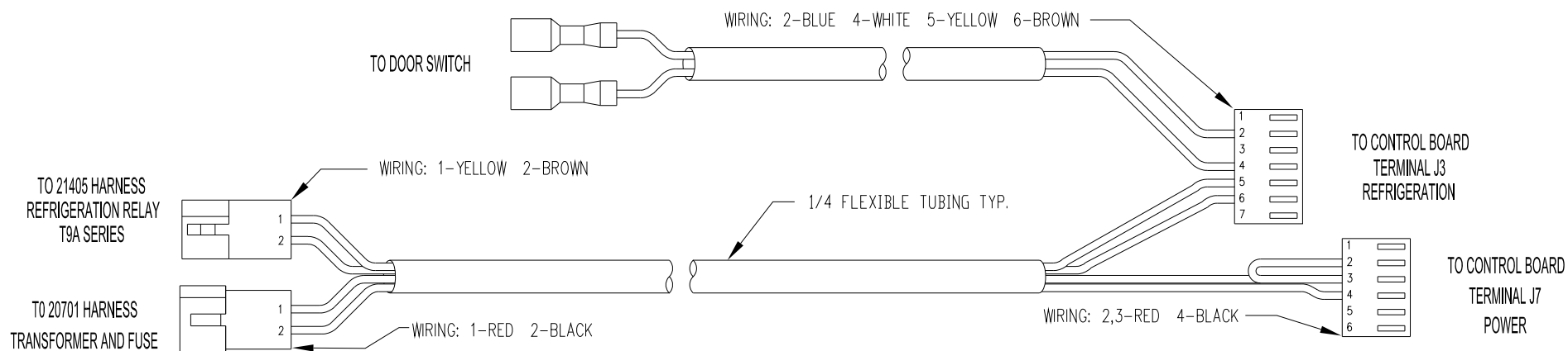
21590, HARNESS, CONTROL POWER AND REFRIGERATION RELAY
