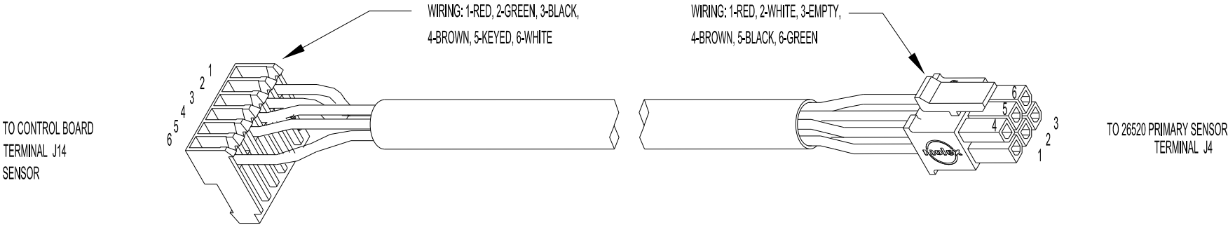
21425 HARNESS, DELIVERY SENSOR DETECTOR/CONTROL
