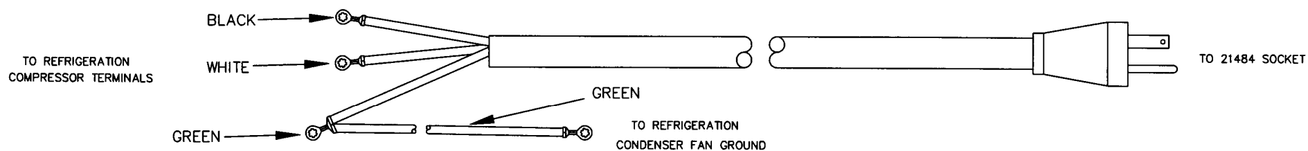
20144, HARNESS, REFRIGERATION
