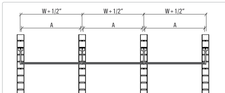
Decorative Bracket
