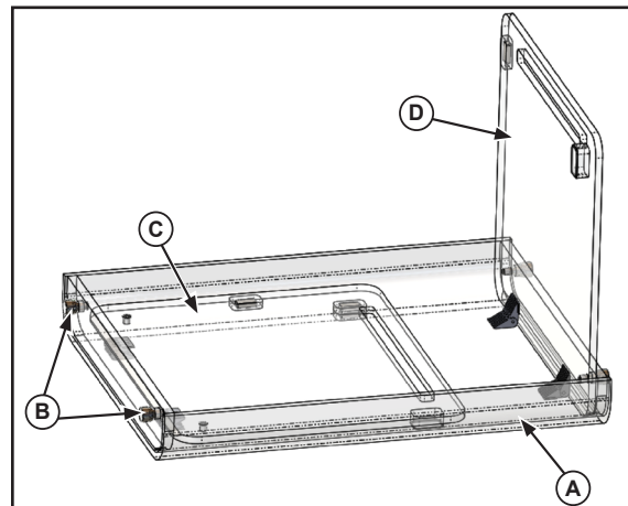
Figure 3. Close Side Panels
