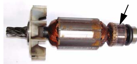
Figure 10: Armature
