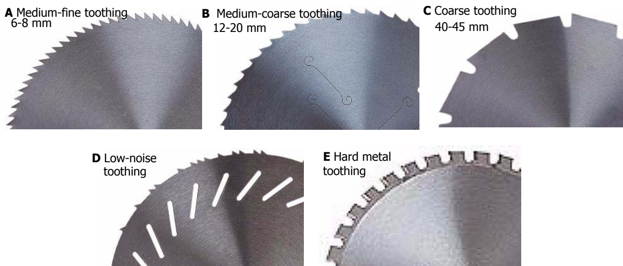
Figure 6: Saw blades
