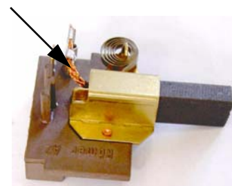
Figure 9: Carbon deposits
