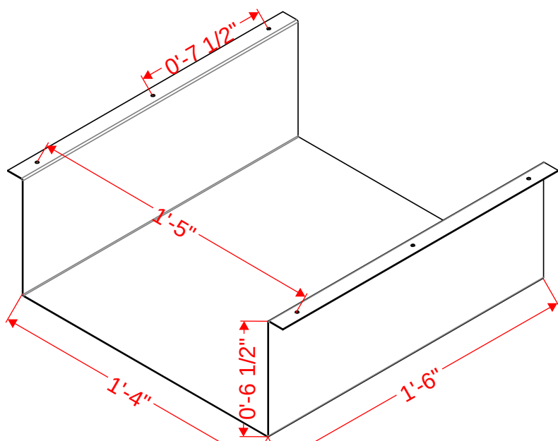
C170190 - Channel Drawer, Hanger Bracket - 1ea.
