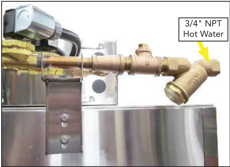
Fig. 6 - Heat recovery hot water connection.
