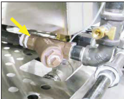
Fig. 10 - Steam inlet.
