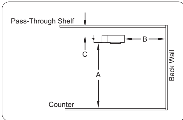
Figure 7. Clearance Requirements
