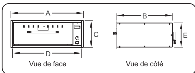
HDW-xBR Dimensions
