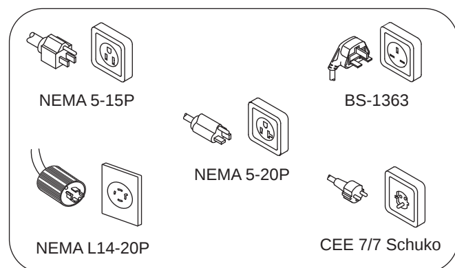
Figure 3. Plug Configurations
