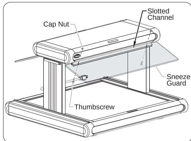
Figure 7. Installing a Sneeze Guard (GR2BW Only)
