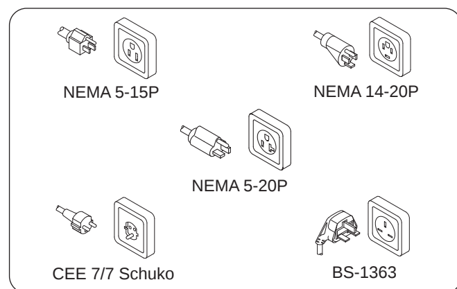
Figure 4. Plug Configurations
