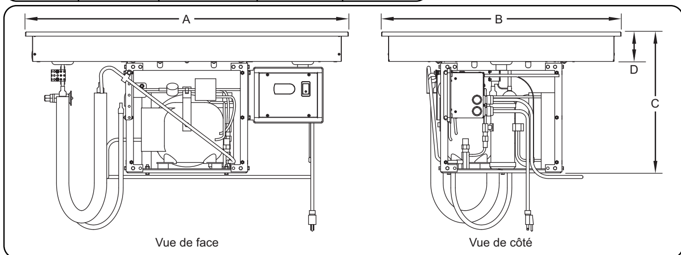
FTB Dimensions
