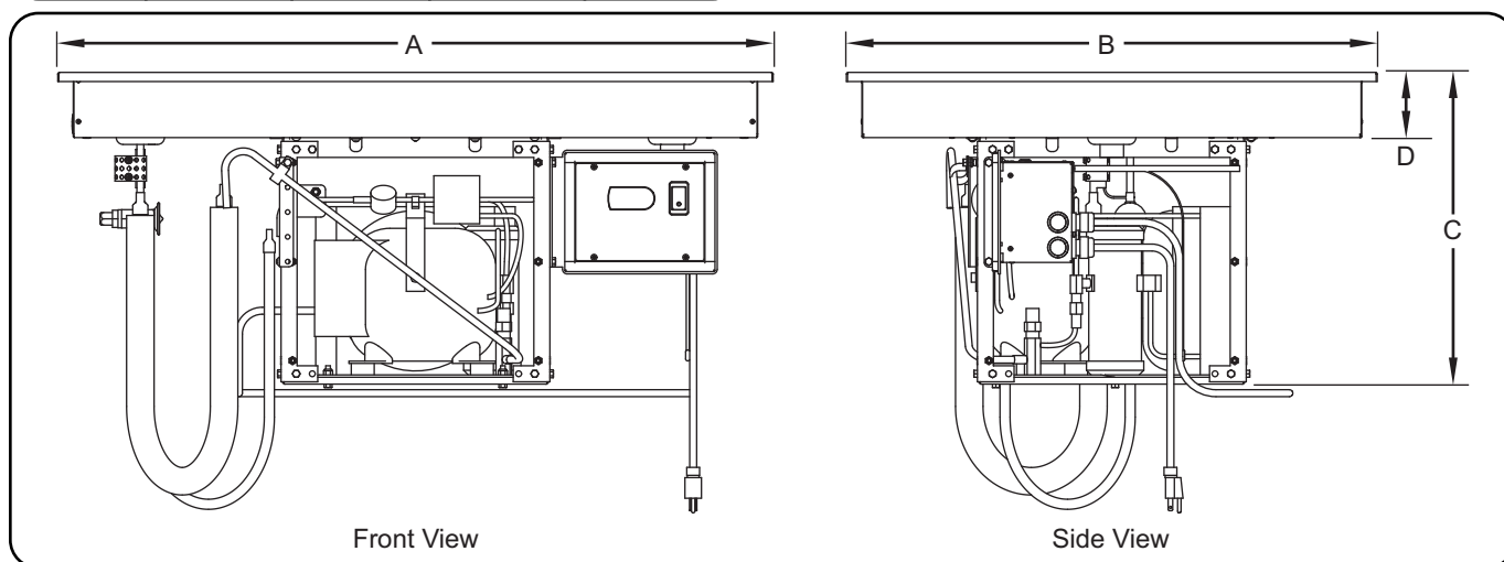
Dimensions—FTB Model
