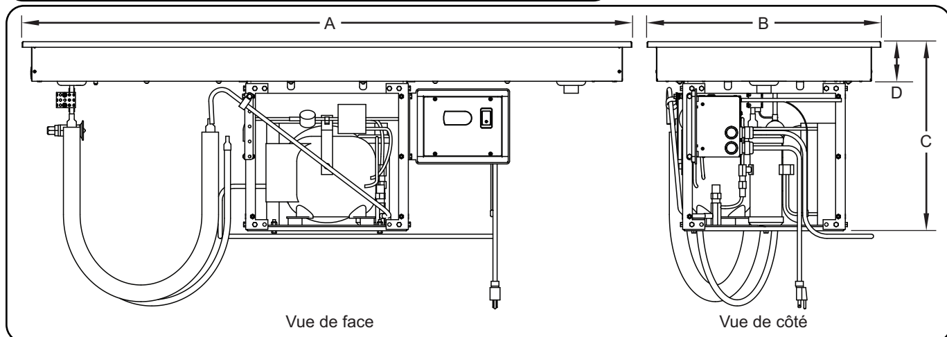
FTB-S Dimensions
