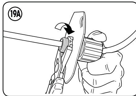
Tighten strain relief nut to the plate with pliers.
