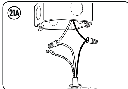
Connect line, neutral and ground per local regulations.
