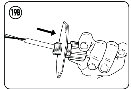
Gently twist strain relief components together - strain relief should still be able to move up and down the cable.
