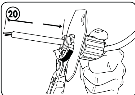
Determine required length of cable and cut allowing 3" that will stick into the electrical box. Tighten strain relief head to secure cord within assembly.
