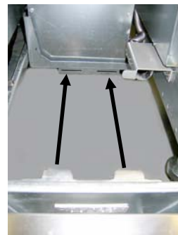
Figure 2: Position the melter in the cabinet and insert tabs into alignment guide slots.
