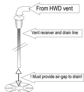
DRAIN VENT DIAGRAM
