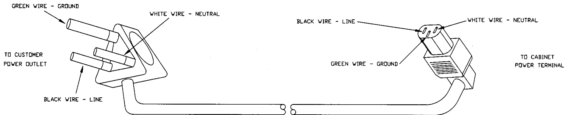
3194, POWER CORD, U.K. & IRELAND
