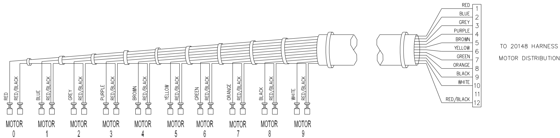
20147, HARNESS, TRAY, 10 COLUMN
