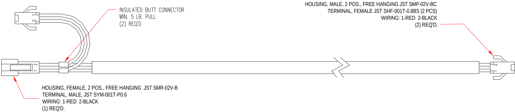
25753 HARNESS, EXTENSION, LED, CLEANLIFE
