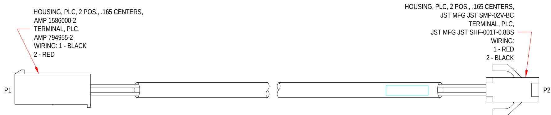
27569 HARNESS, ASSEMBLY, LED EXTENSION / ADAPTOR CLEANLIFE
