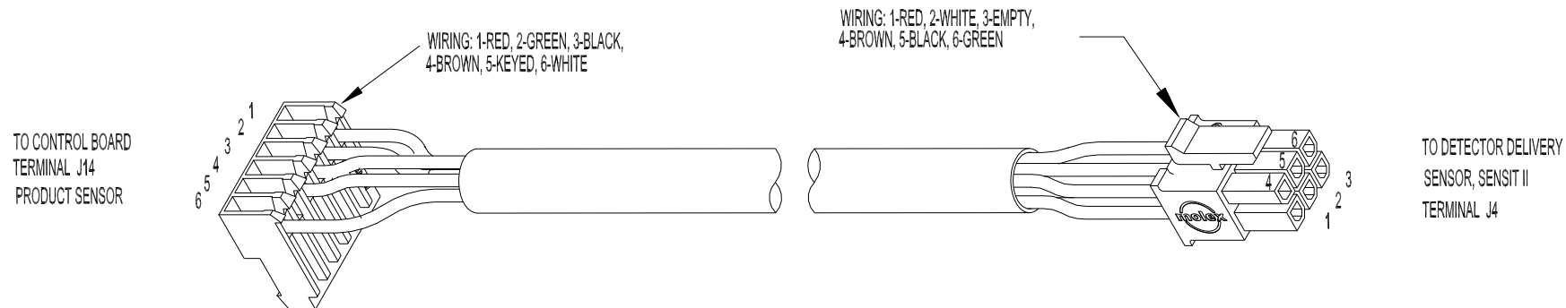
23503 HARNESS, DELIVERY SENSOR DETECTOR/CONTROL, SENSIT II
