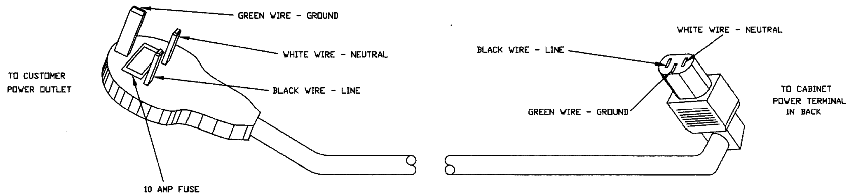
3194, POWER CORD, U.K. & IRELAND
