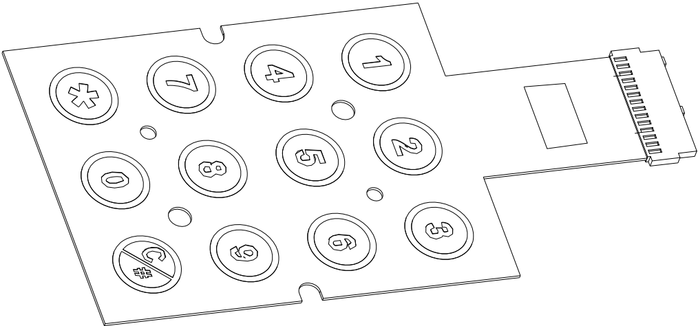
25688 ASSEMBLY, LIGHTED KEYPAD
