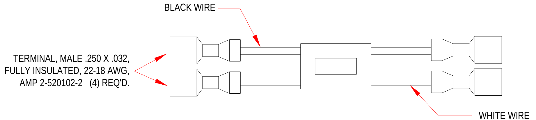
25494 RFI, FILTER BYPASS
