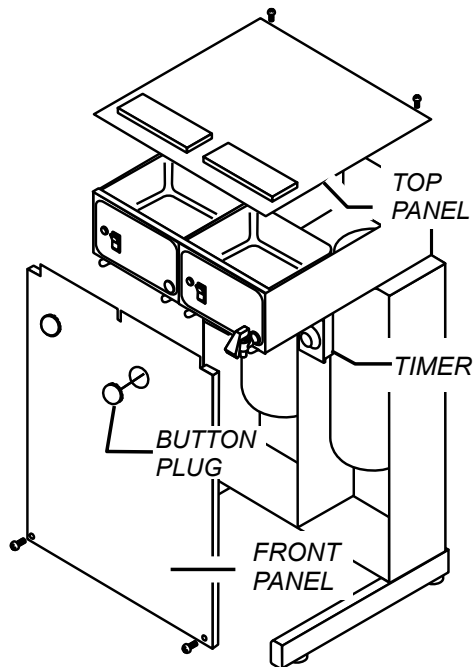
Fig. 9 Access Panels
