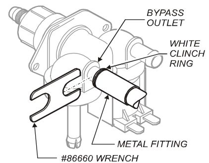
P/N 86660 Braided Hose Wrench
