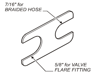
P/N 86660 Braided Hose Wrench
