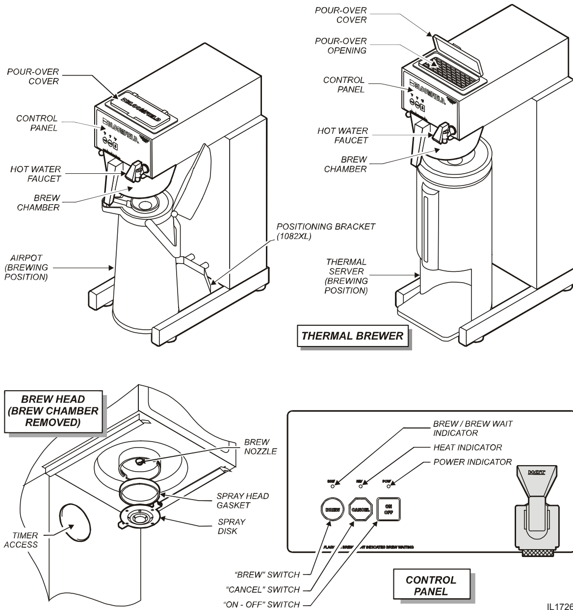
Fig. 1 Features & Operating Controls
