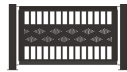
BAND PATTERN MF5054 14 1/2" X 2" X 32" 15 lbs. - Quarter Panel MF5050 25 1/2" X 2" X 32" 22 lbs. - Half Panel MF5046 55" X 2" X 32" 40 lbs. - Full Panel Posts sold separately
