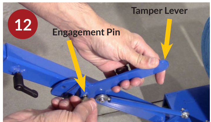
Step 12: Lean cart back and pull the pin. Push lever forward until it locks in bottom hole. This disengages roller.
