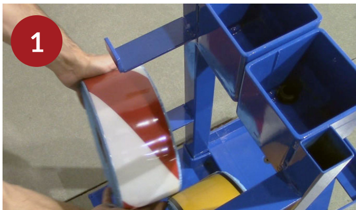
Step 1: Load 4" Tape (if applicable) on lower hooks of tape holder.
