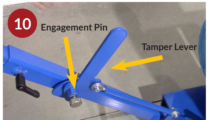
Step 10: Lean cart back and pull engagement pin. Handle will come toward you until pin locks in upper hole.
