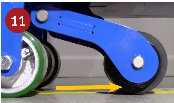
Step 11. Once tamper roller is on floor, push Kaizen Cart back and forth over the area several times to ensure proper adhesion.
