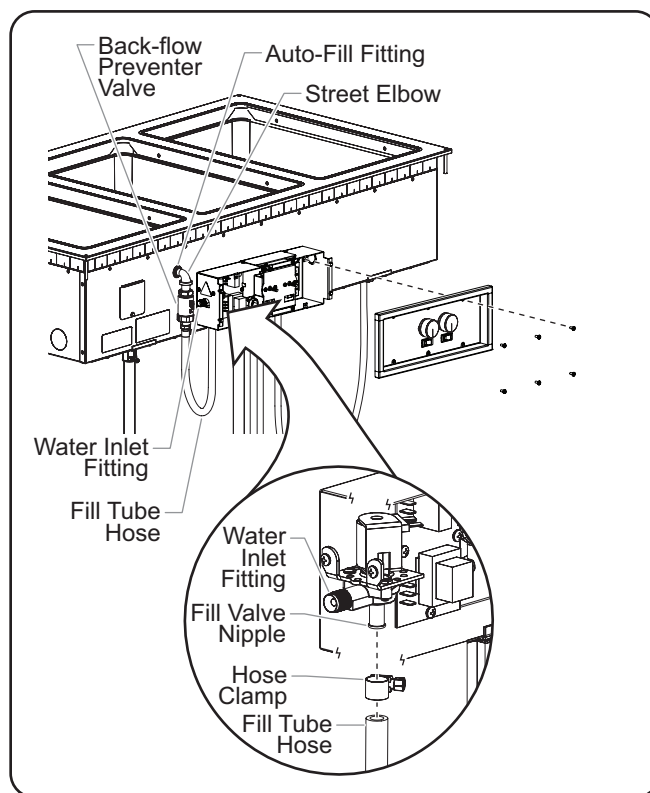
Installing a Side Mounted Auto-Fill Unit
