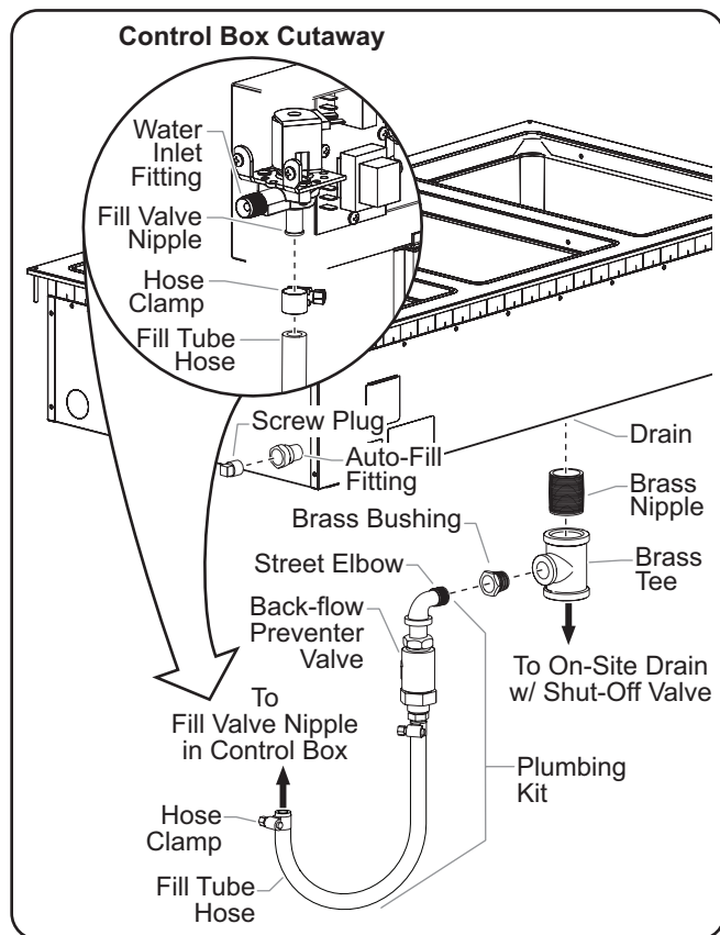
Installing a Drain Mounted Auto-Fill Unit
