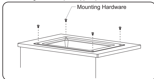
Through-Hole Mounting
