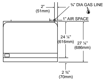
Standard Griddle
