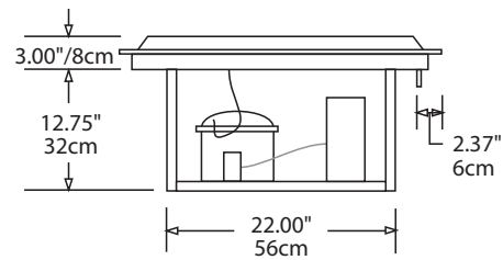
Right End View N8200 Models
