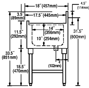
side view dimensions of all 1800 Series underbar sinks
