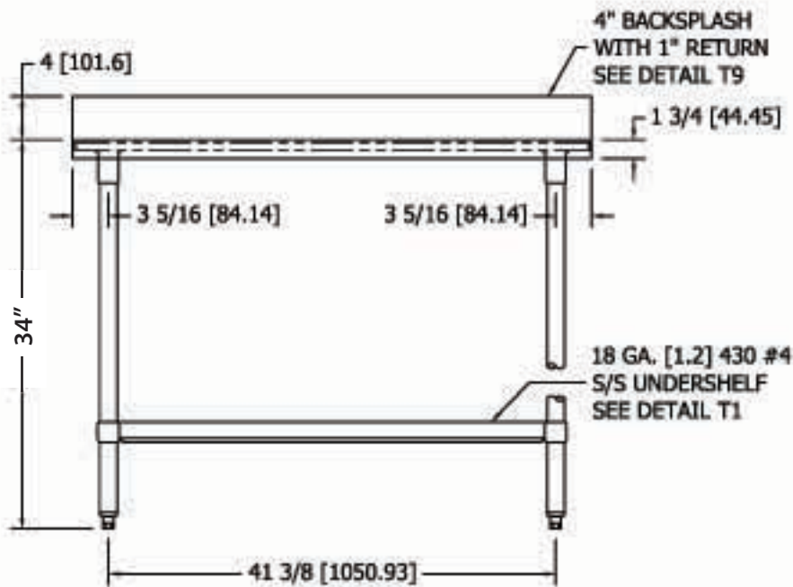
FRONT ELEVATION
