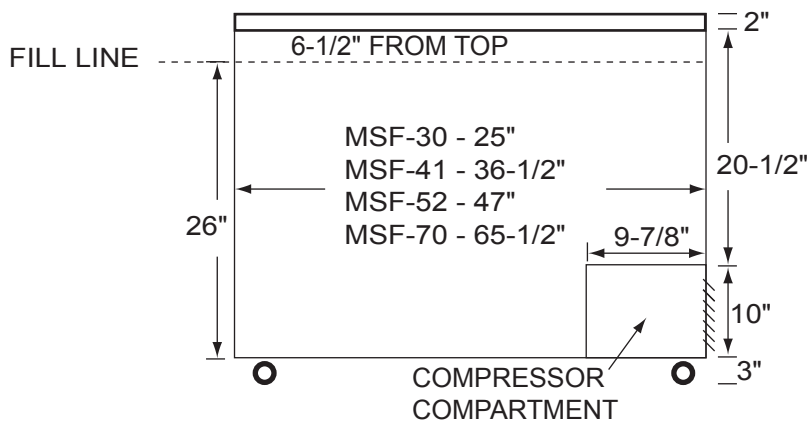
ELEVATION VIEW
