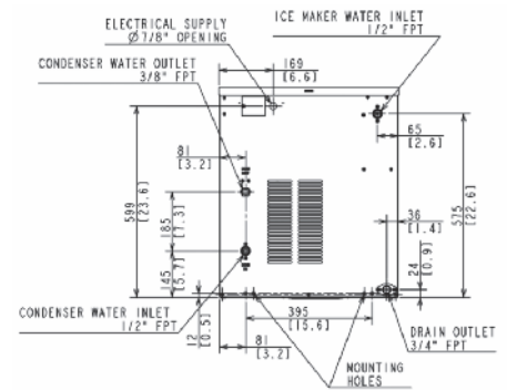
WATER-COOLED UNIT
