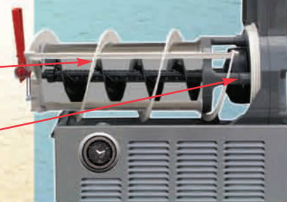
Cut-Away View
