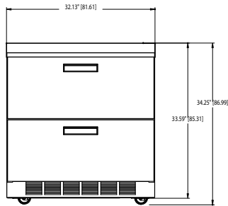
UCD4532N Elevation View
