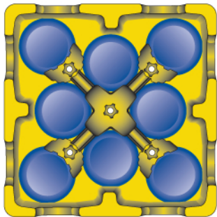
ADS4 Layout for 7-1/2" plates
