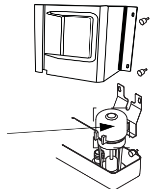
Water Pump Removal
