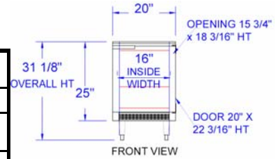
UCR/UCF20 FRONT
