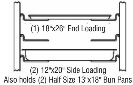
LOADING CAPACITY
