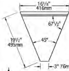
#MF45-18 Front Filler
