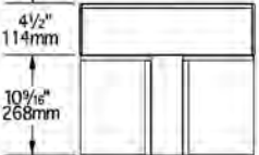
#MR45-18 Rear Filler
