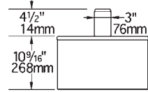
#MF45-18 Front Filler
