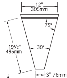
#MF30-18 Front Filler
