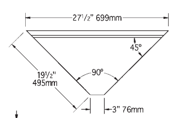
#MF90-18 Front Filler
