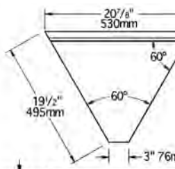
#MF60-18 Front Filler
