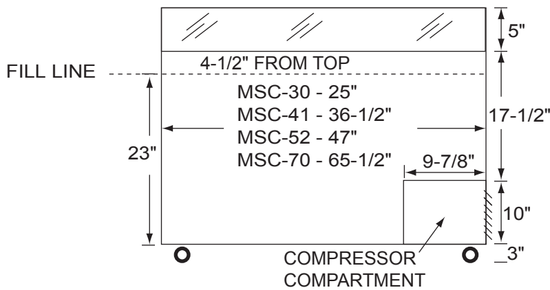
ELEVATION VIEW
