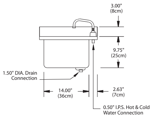
Elevation View
