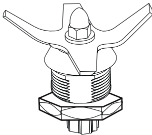
030857 Blending Assembly ONLY (with hex nut and washer)
