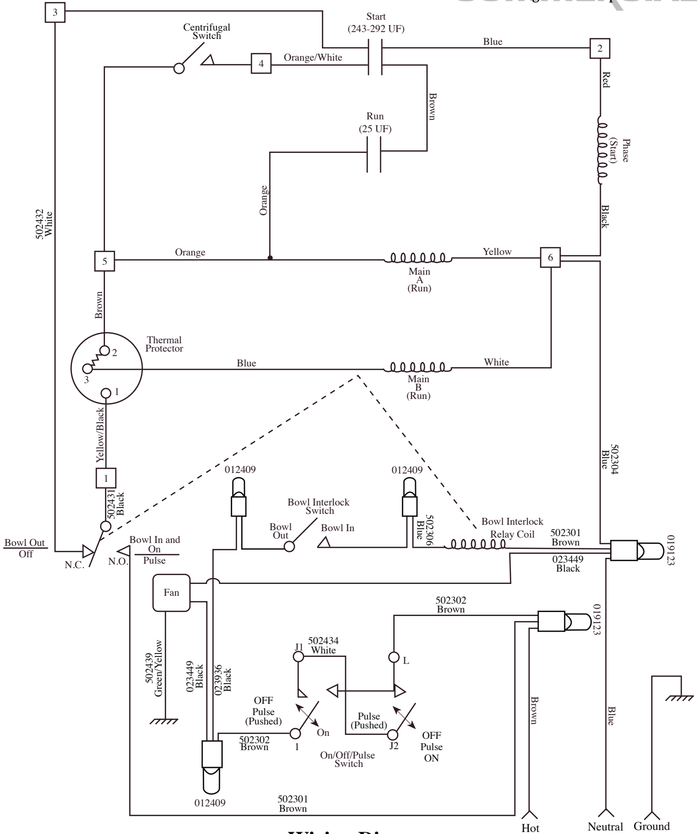
Wiring Diagram
